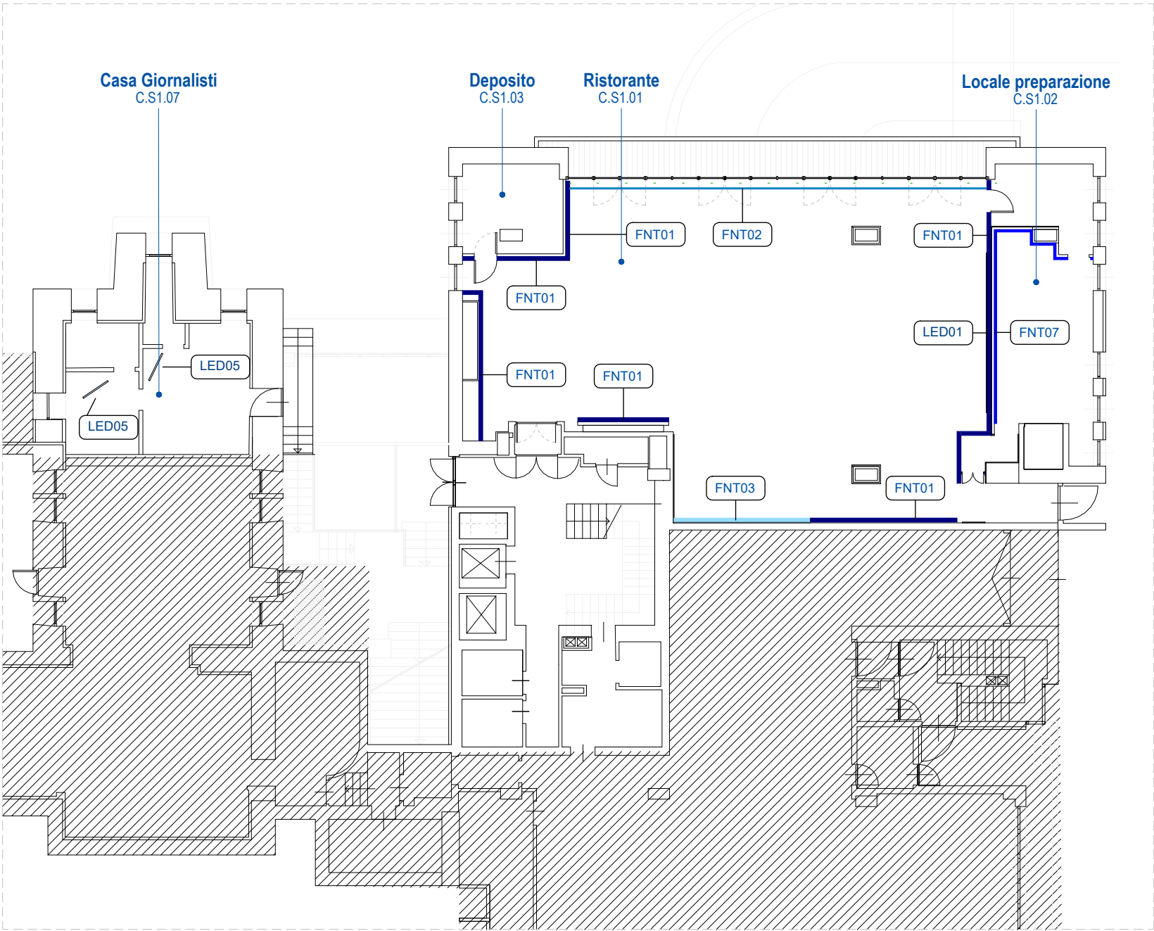
PIANTA PS1 - ABACO FINITURE VERTICALI 1 : 200
